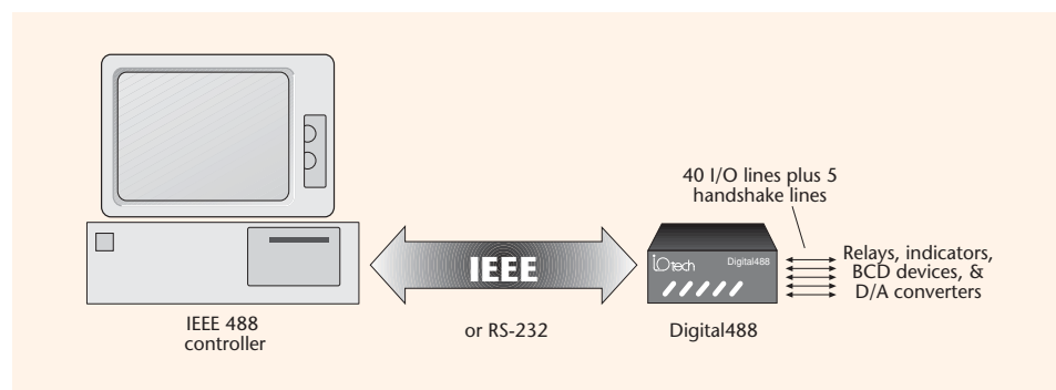
Digital488 provides an economical link between an IEEE 488 controller and digital signals
